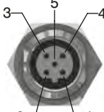
M12 5P FEMALE
